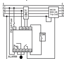
Failsafe Mode with Uv Trip Coil
