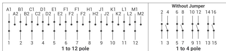
Connection Diagram
