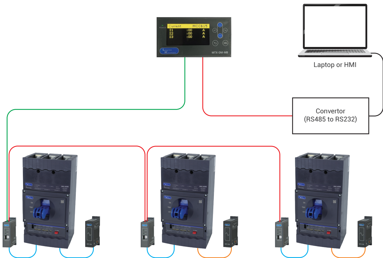
MODBUS Communication through MODBUS looping
