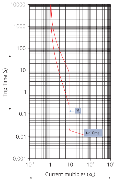
DN0 MCCB
