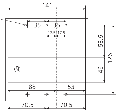
Mounting & Door Cut-out Details
